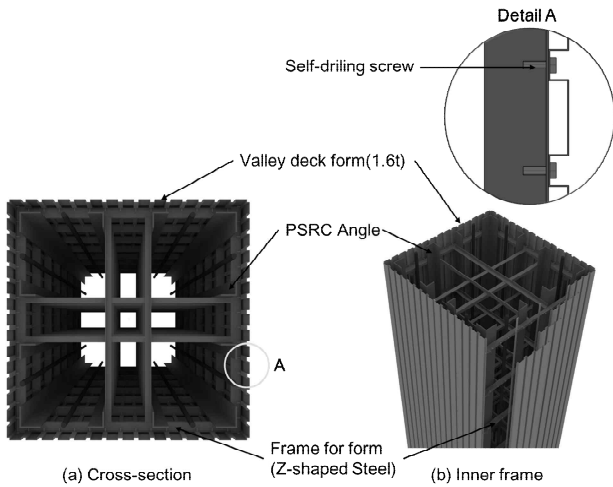
Figure 3. Form-LPSRC column
