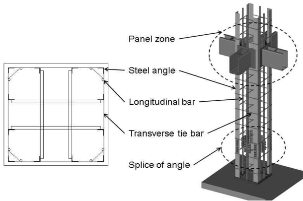
Figure 2. PSRC column
