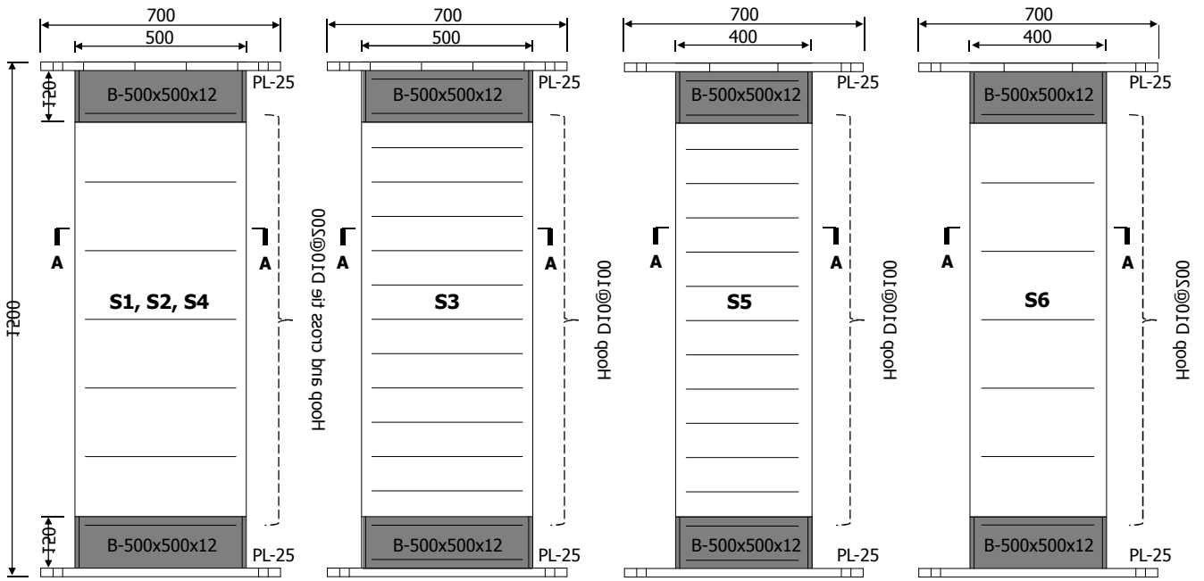
(a) Spacing of lateral reinforcement
