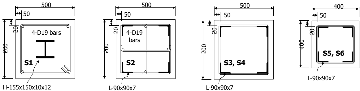
(b) Details of structural steel and reinforcing bars (cross-section A-A)
