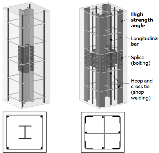
(a) Existing SRC column (b) Prefabricated SRC (PSRC) column
